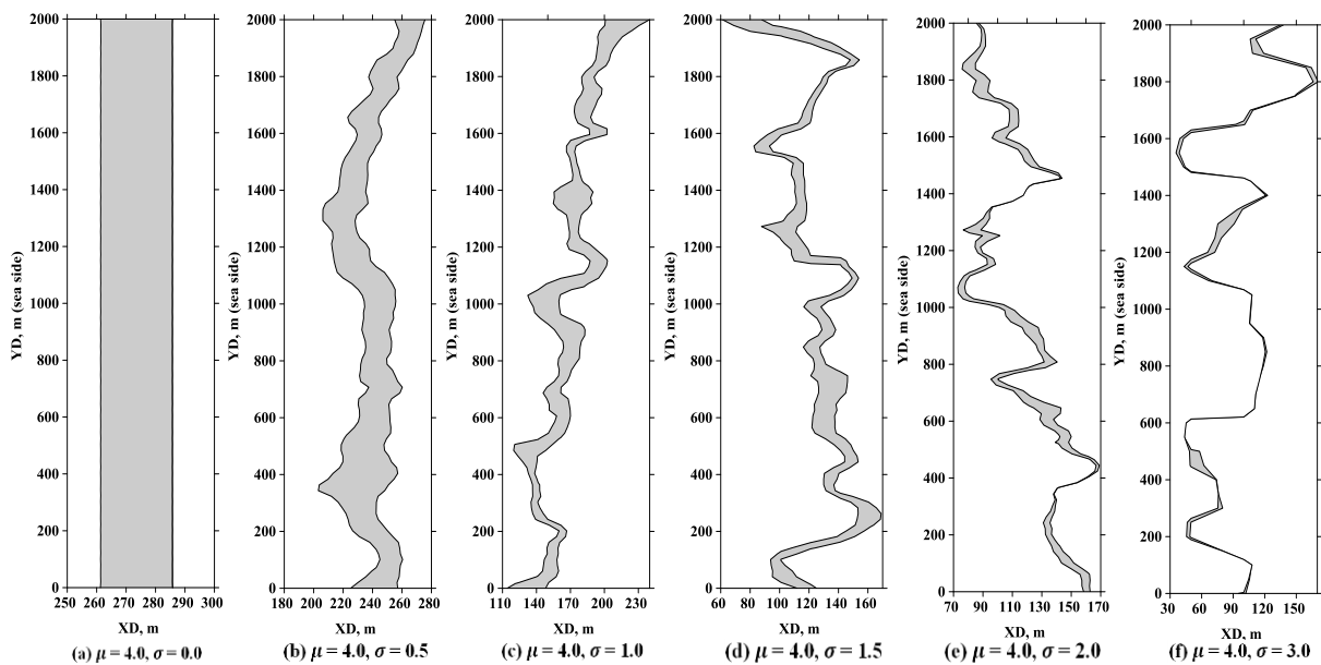
Figure 10: Variation of interface toe distance at different cross sections for every case of heterogeneity
