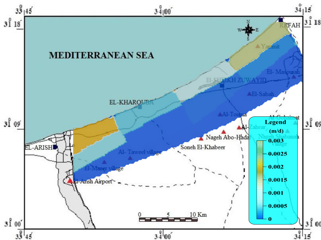
Figure 15: Calibrated recharge Zones
