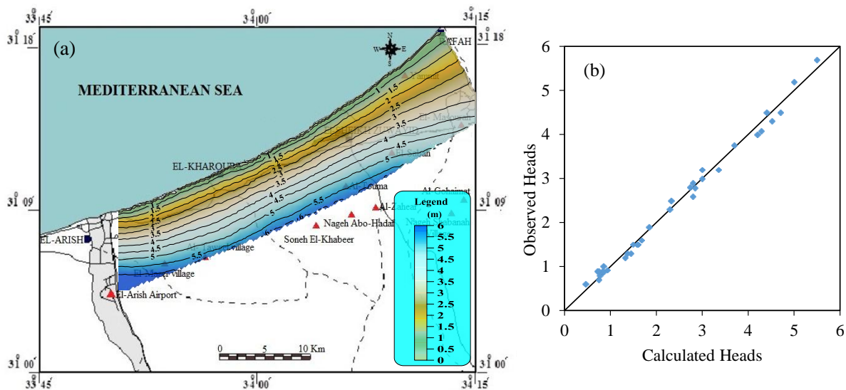
Figure 17: Contour lines of the calculated heads, and a comparison of calculated and observed heads
