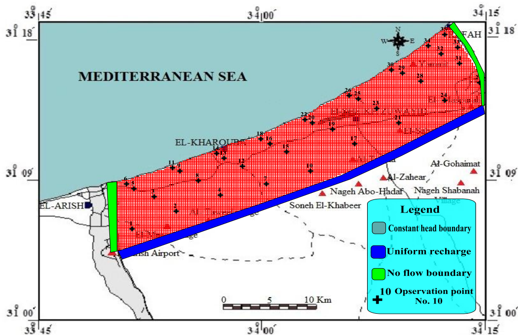
Figure 14: The grid of the studied domain for Quaternary aquifer and the used boundary conditions
